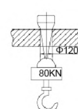
Detail B
