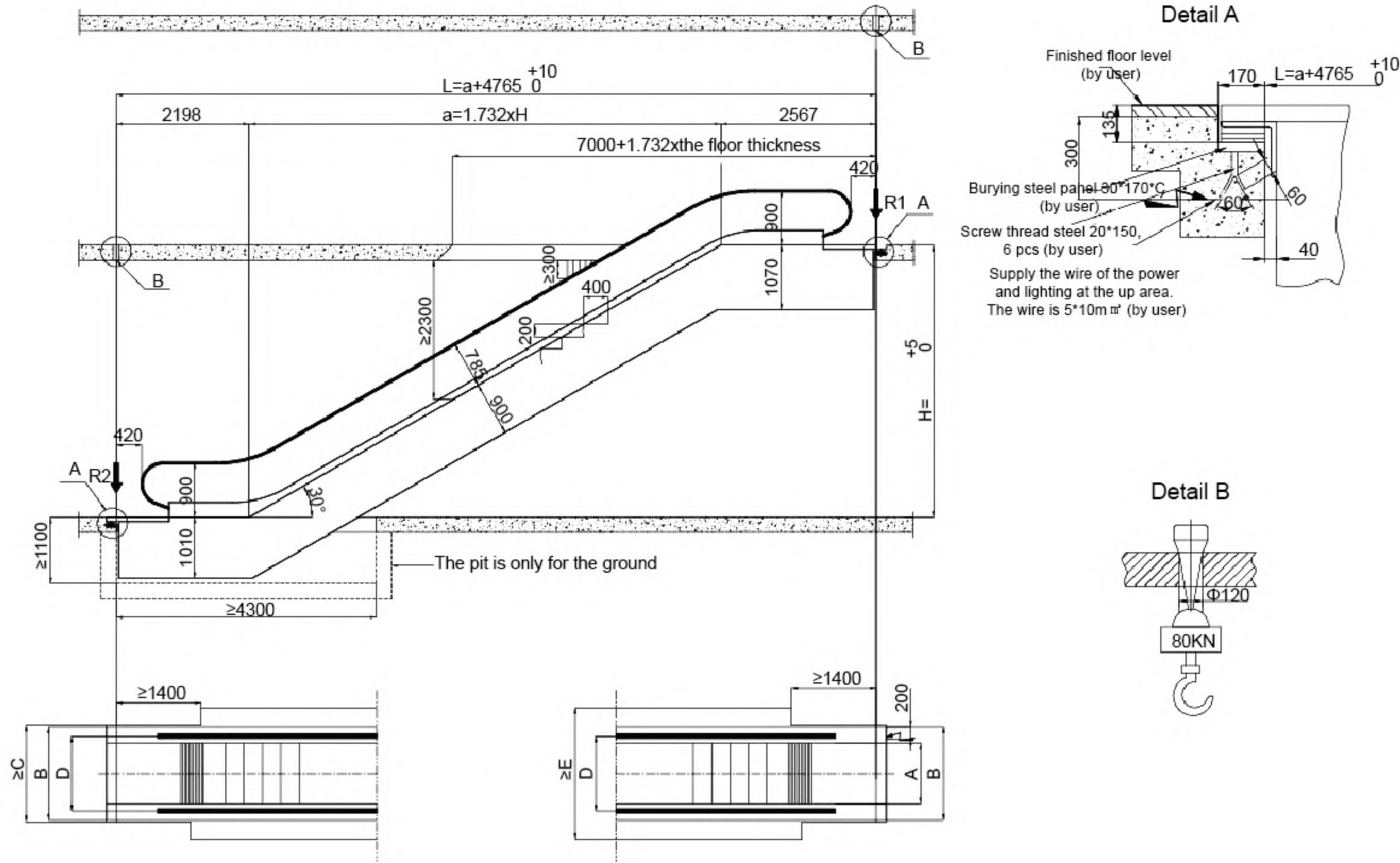
Reacting force
